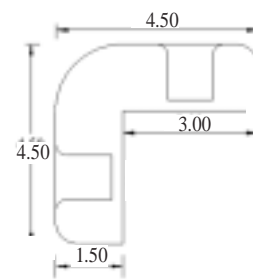
Side View Part #441
